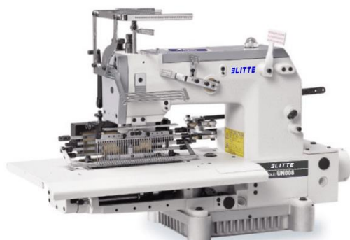
UN008-33048P/VPQ/VSM 多针双链式环缝机 (单根橡筋线缩褶打缆) Multi-needle double-chain circular sewing machine (Single elastic shirring smocking) (elastic up/no bottom thread; smocking function)
